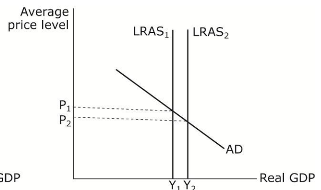
Classical long-run AS curve
