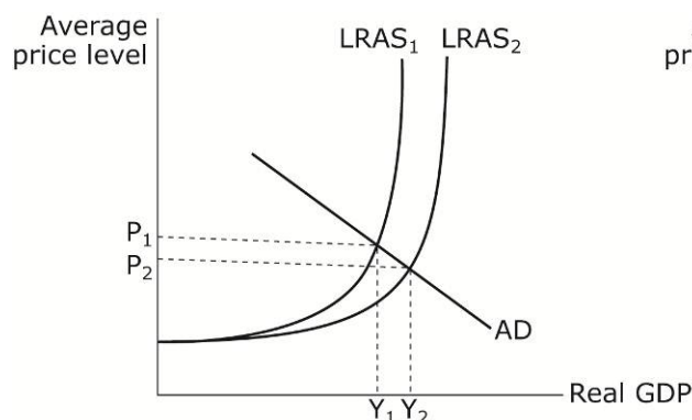
Keynesian long-run AS curve
