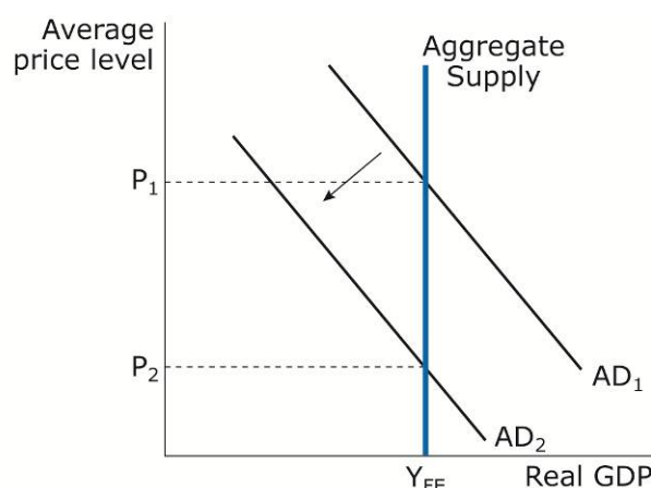
Classical LRAS curve
